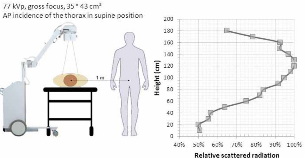
Figure 4. Variation of scattered radiation in relation to the height of the exposed worker for configuration 1
